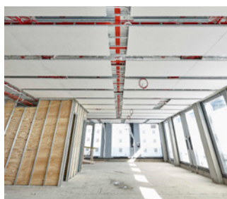
Chilled Ceiling
